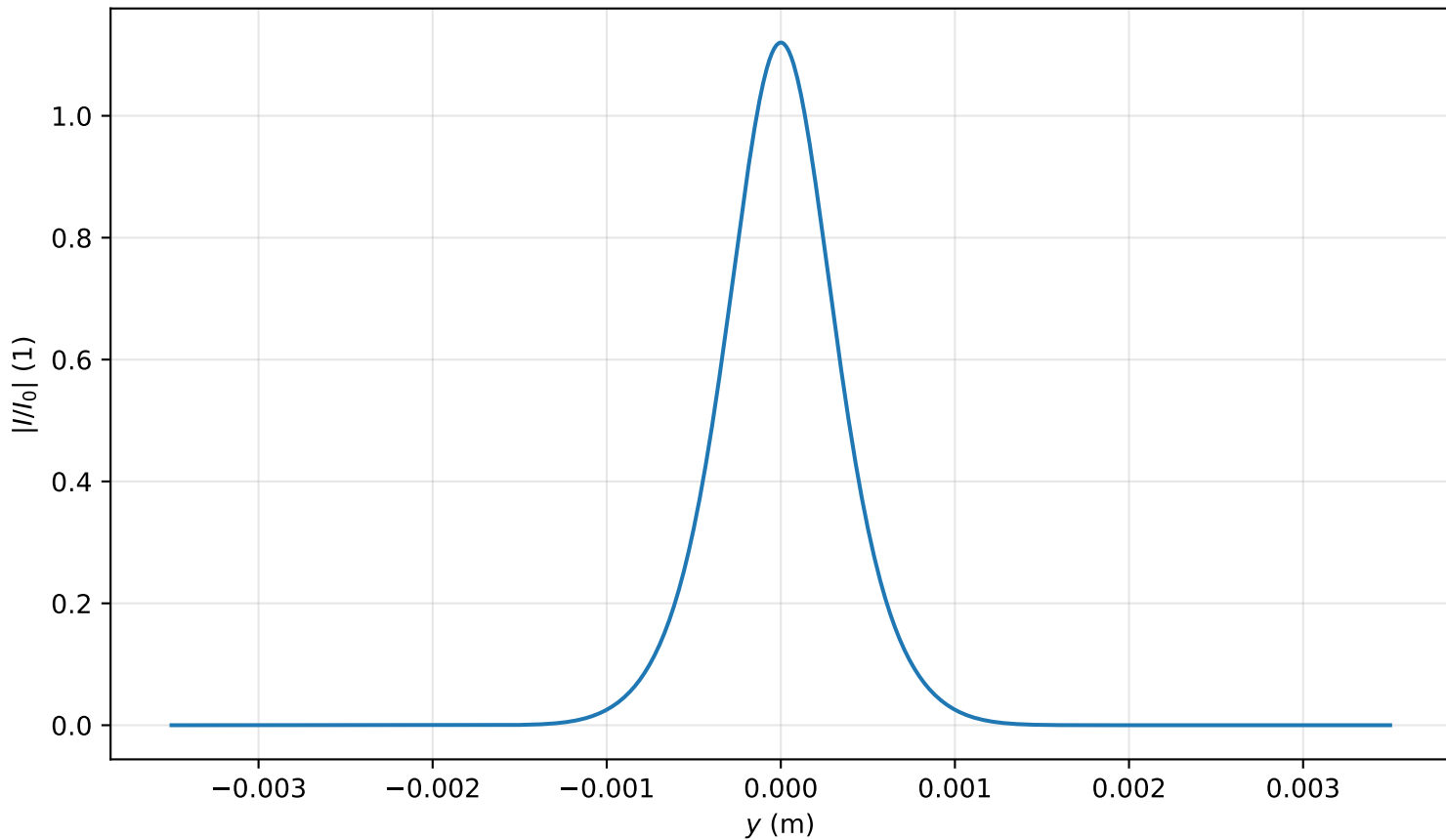
Intensity profile I(x=0, y, z=0.955)/I_0 , P_{in}=0.6P_{cr} , artificial time
